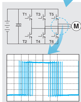
Figure 1.2.4 Inverter PWM output waveform
