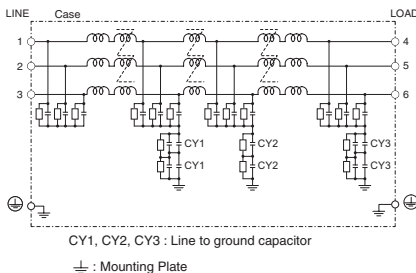
(3) Line to ground capacitor code : 136
