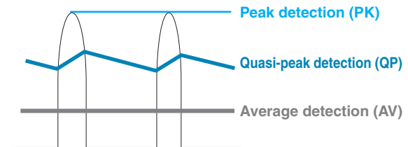
Figure 5.13.1 Relations between Detection Methods and Measurement Levels
