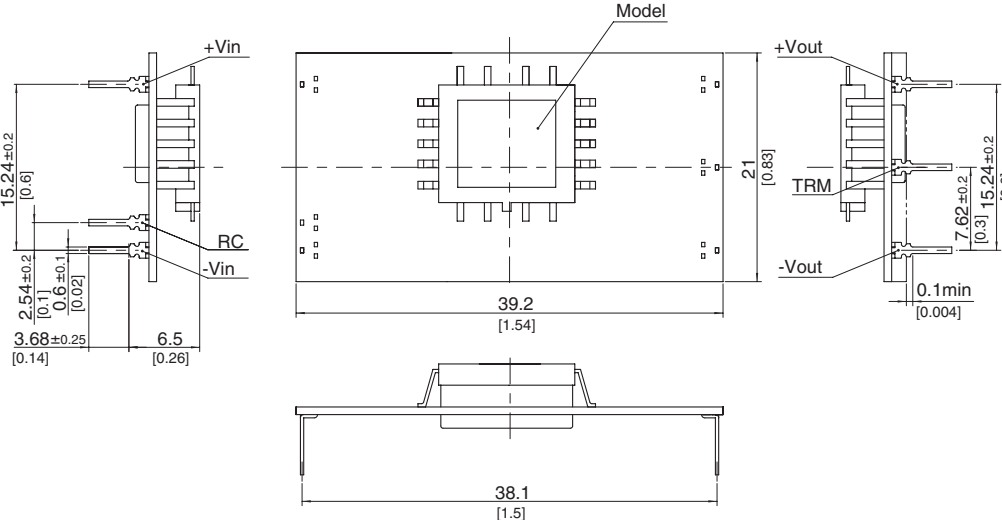
2. DIP(type C)
