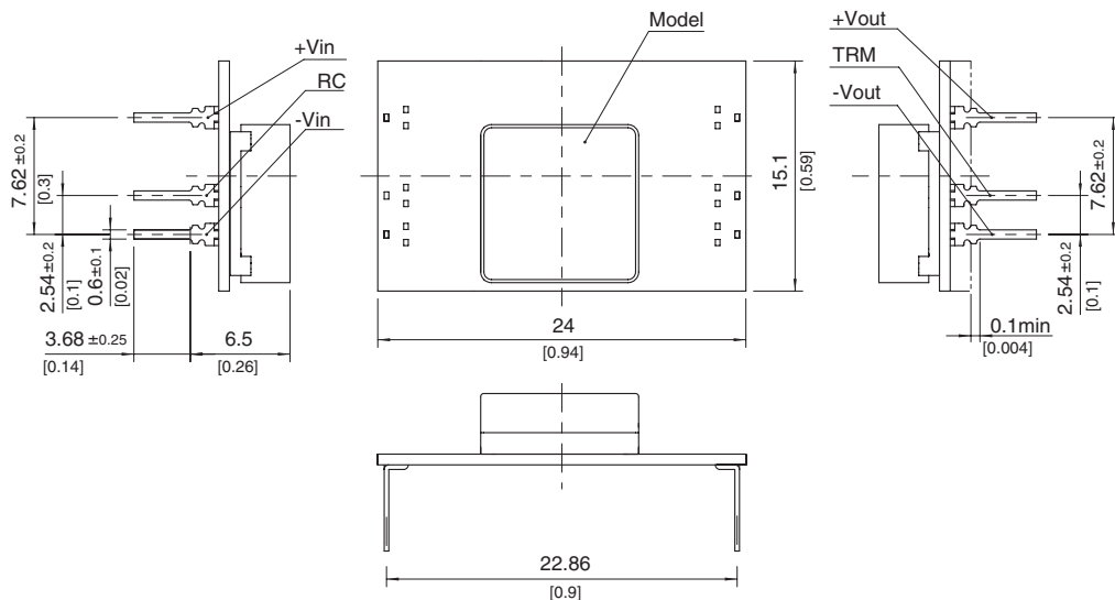
2. DIP (type C)
