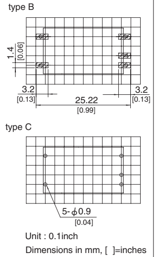
Recommended Pad and Hole dia. (TOP VIEW)
