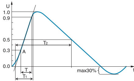
Figure 5.8.1 Example of a Surge Waveform in Voltage
